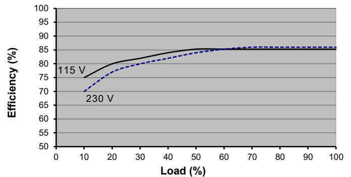
(Model DPGRN45-3001 Efficiency shown)
