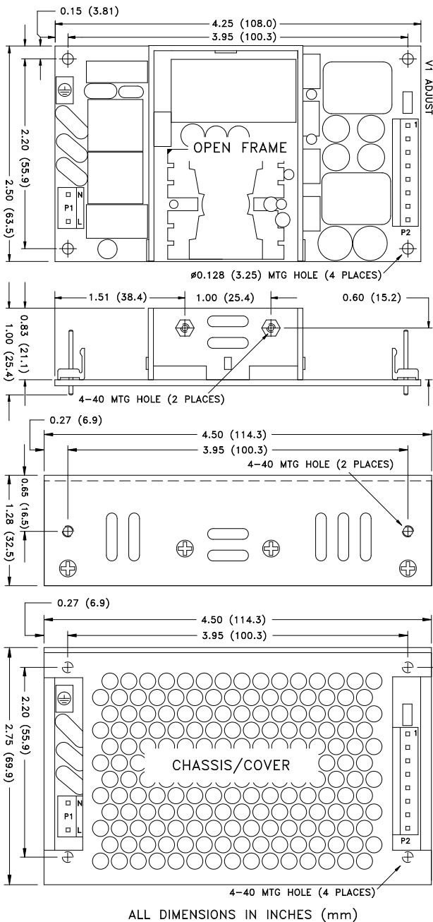
ALL DIMENSIONS IN INCHES (mm)
